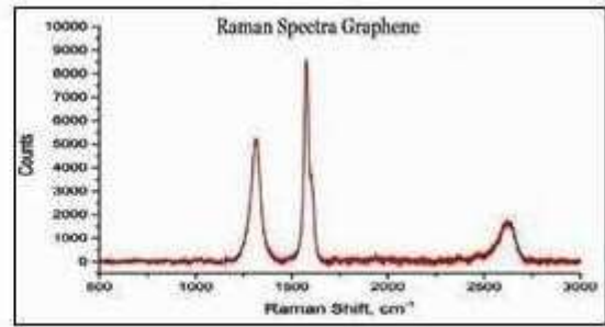
RAMAN Spectrum
