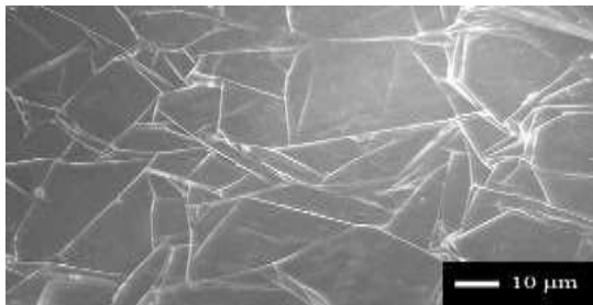
SEM image of Graphene Sheet
